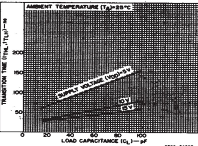
Fig.11 – Typical transition time as a function of load capacitance.
