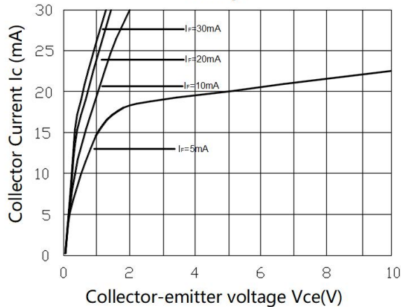
Fig.3 Collector Current vs. Collect-emitter voltage
