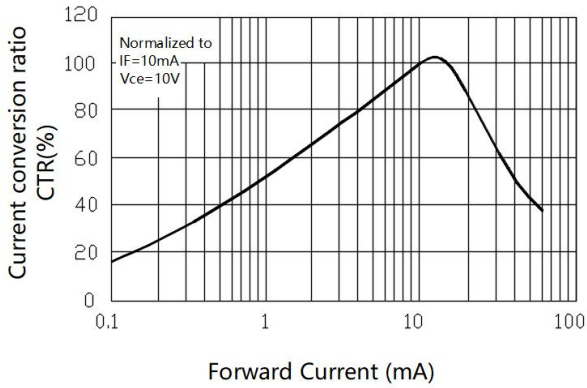
Fig.1 Relative Current Transfer Ratio vs. Forward Current
