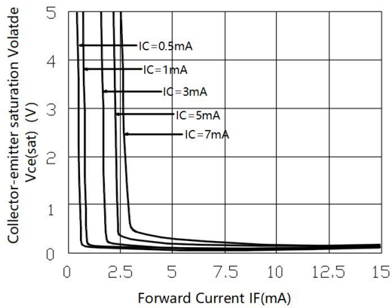
Fig.9 Collect-emitter Saturation Voltage vs. Forward Current
