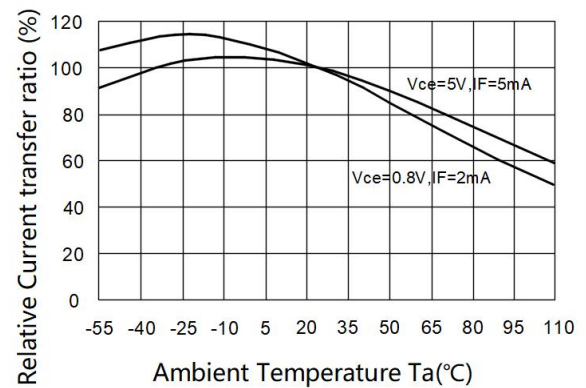
Fig.4 Relative Current Transte vs. Ambient Temperature
