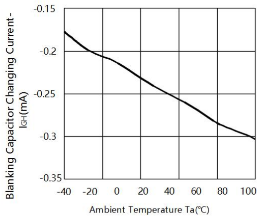
Fig.11 Blanking Capacitor Changing Current vs. Ambient Temperature
