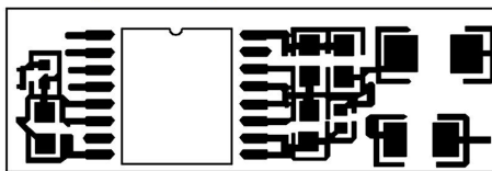
Minimum Components placed on one sides
