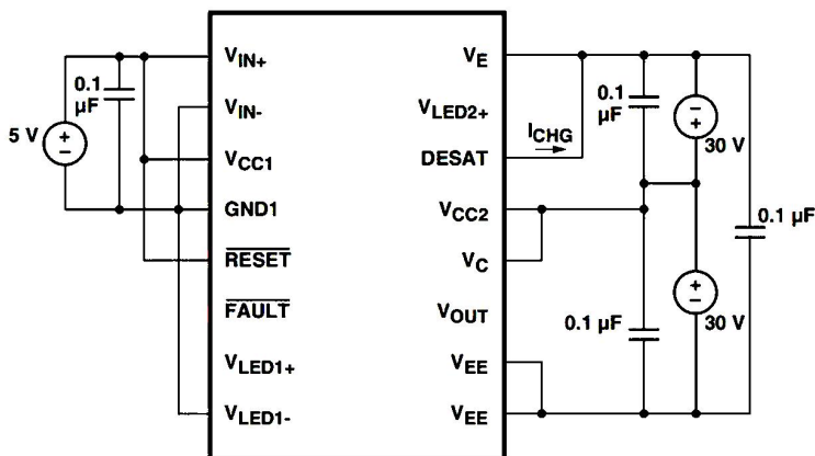
Fig35. ICHG pulsed test circuit
