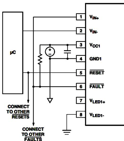
Figure 67a. safe hardware reset for noninverting input configuration (automatically resets for every
