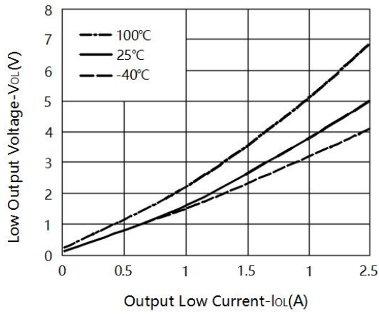
Fig.7 Low Output Voltage vs. Output Low Current
