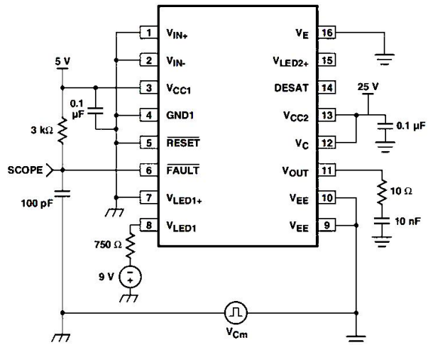
Fig48. CMR test circuit,LED1 on
