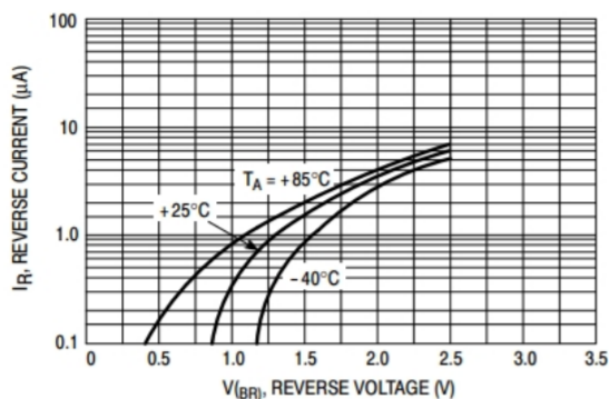
Reverse Characteristics
