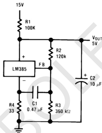
Low AC Noise Reference
