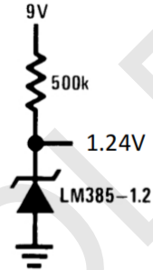
Micropower Reference from 9V Battery
