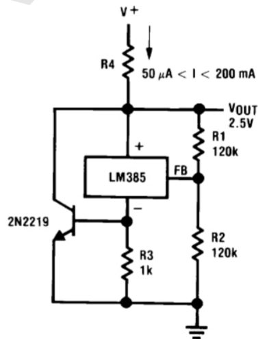
200 mA Shunt Regulator
