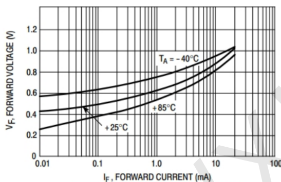
Forward Characteristics
