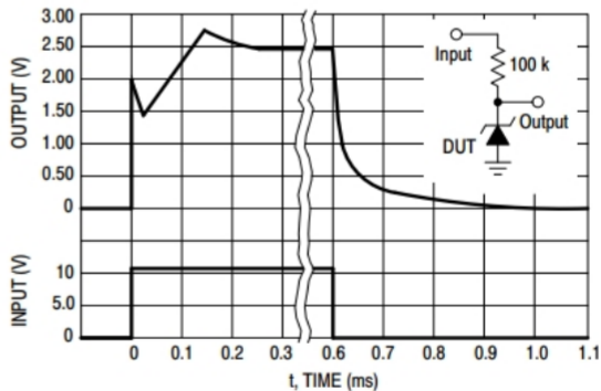
Response Time
