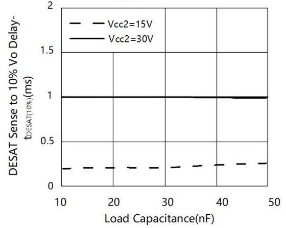
Fig.20 DESAT Sense to 10% Vo Delay vs. Load Capacitance
