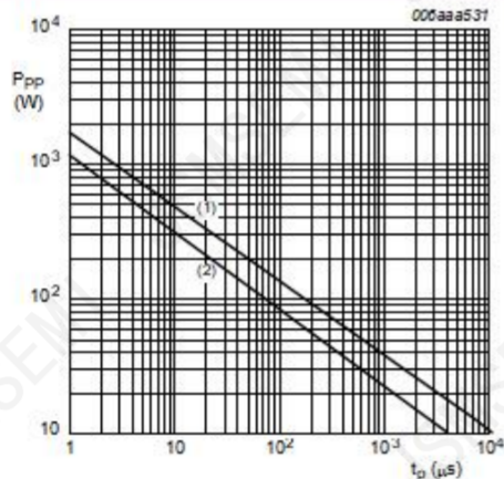
T_{amb} = 25\text{ }^{\circ}\text{C} (1) PESD3V3L2BT and PESD5V0L2BT (2) PESD12VL2BT, PESD15VL2BT, PESD24VL2BT Fig 3. Peak pulse power as a function of exponential pulse duration t_p ; typical values
