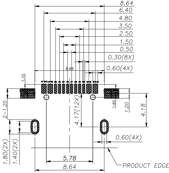
RECOMMENDED PCB LAYOUT(TOP VIEW) THICKNESS 0.80MM:DEFAULT TOLERANCE:±0.05
