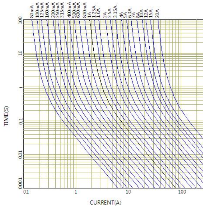
I-T CURVE
