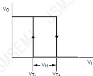
Figure 6. Transfer characteristic
