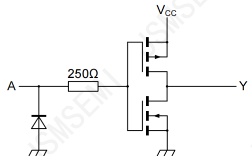
Figure 3. Logic diagram (one gate)
