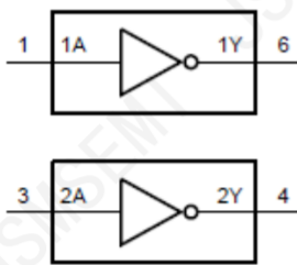
Figure 1. Logic symbol
