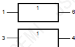
Figure 2. IEC logic symbol
