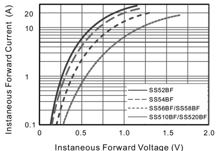
Fig.3 Typical Forward Characteristic
