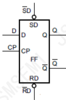
Figure 1. Logic symbol
