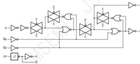
Figure 3. Logic diagram
