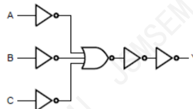
Figure 3. Logic diagram
