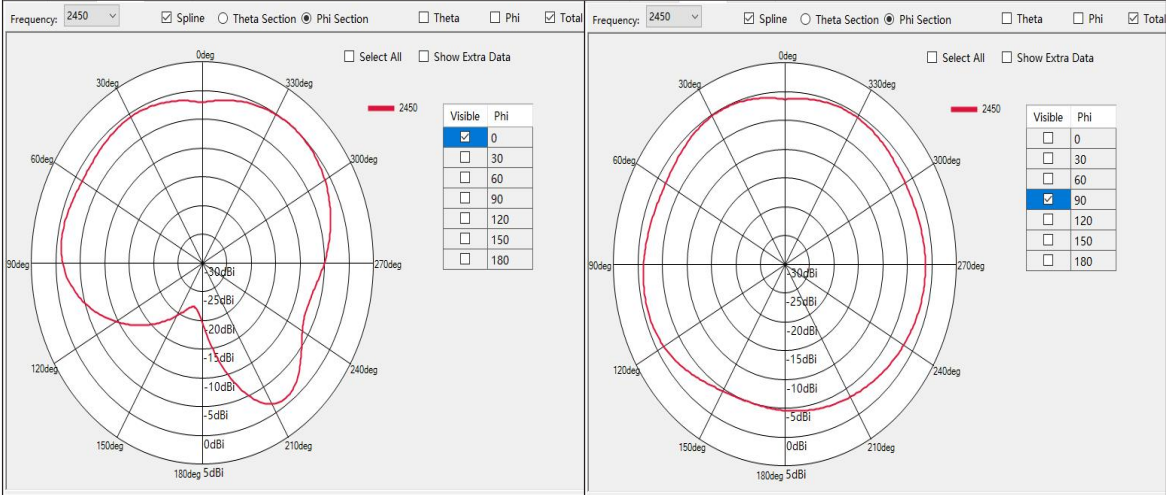
\phi = 0^\circ Plane XZ at 2450 MHz, Gain 0.22 dBi
