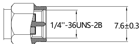
DETAIL A SCALE 2:1
