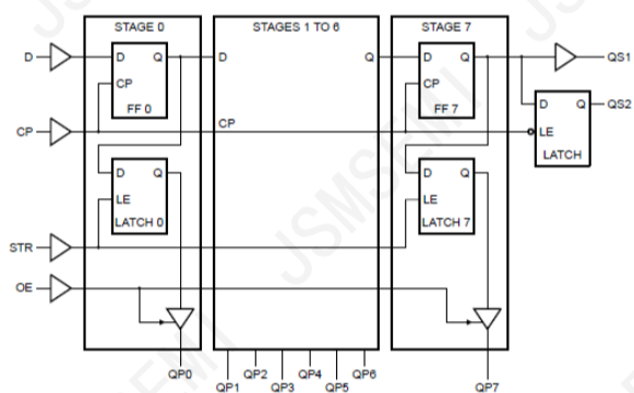
Figure 3. Logic diagram
