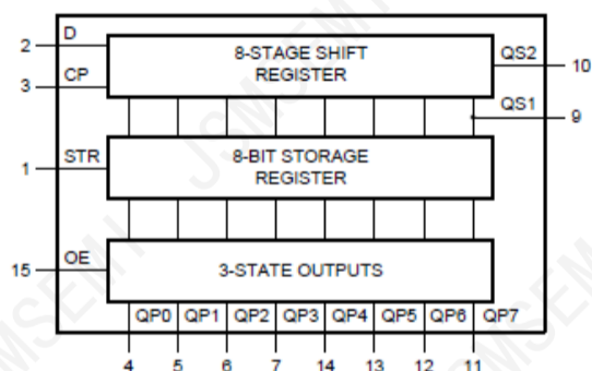
Figure 2. Functional diagram
