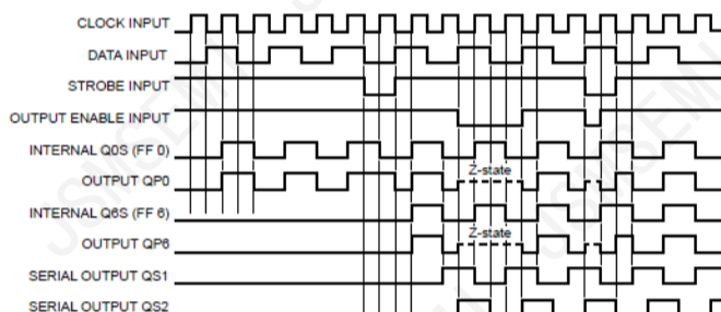
Figure 4. Timing diagram
