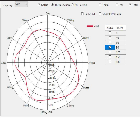
\theta = 90^\circ Plane XY at 2450 MHz, Gain 2.64 dBi
