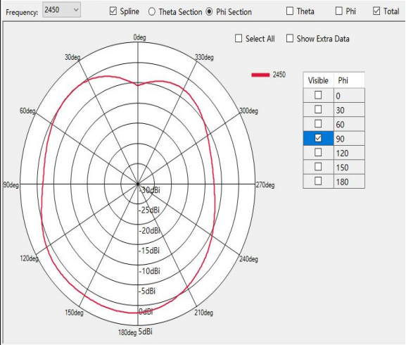
\phi = 90^\circ Plane YZ at 2450 MHz, Gain 2.64 dBi
