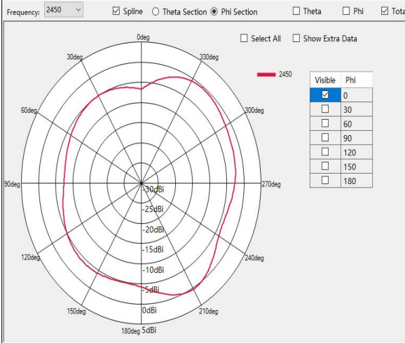
\phi = 0^\circ Plane XZ at 2450 MHz, Gain 2.64 dBi
