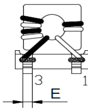
侧视图 Side view
