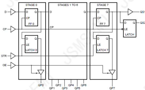
Figure 3. Logic diagram
