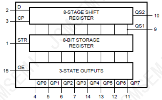
Figure 2. Functional diagram
