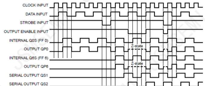
Figure 4. Timing diagram
