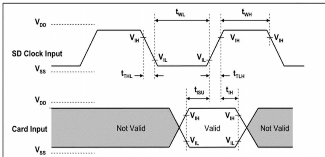
SDIO device input timing(Default Speed Mode)
