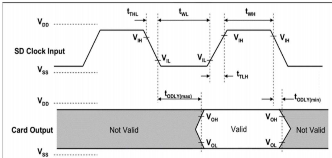
SDIO device output timing (Default Speed Mode)
