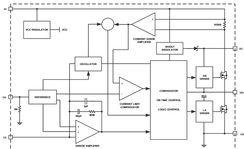
ADP2301AUJZ-R7-MS Block Diagram
