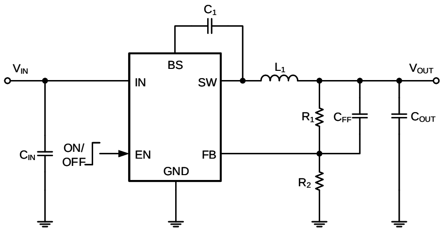
BasicApplication Circuit
