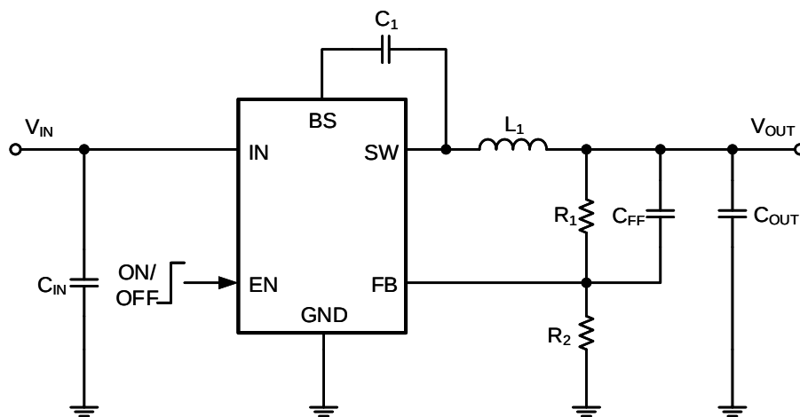
BasicApplication Circuit
