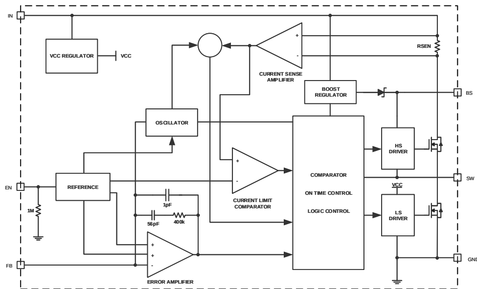
AOZ1280CI-MS Block Diagram
