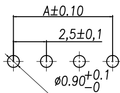
SUGGESTED PCB LAYOUT (COMPONENT SIDE)
