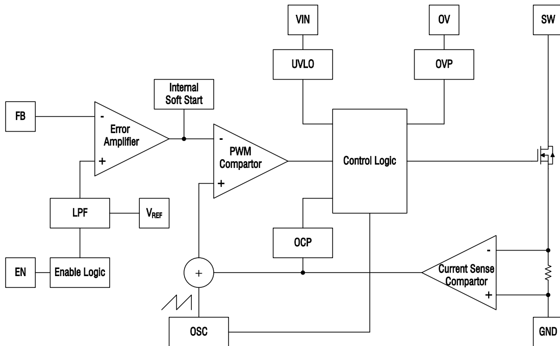
Figure 2. MP3202DJ-LF-Z-MS Block Diagram
