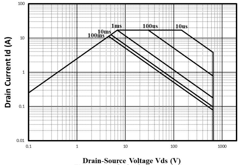
Drain-Source Voltage V_{ds} (V) Figure 18. Safe Operating Area
