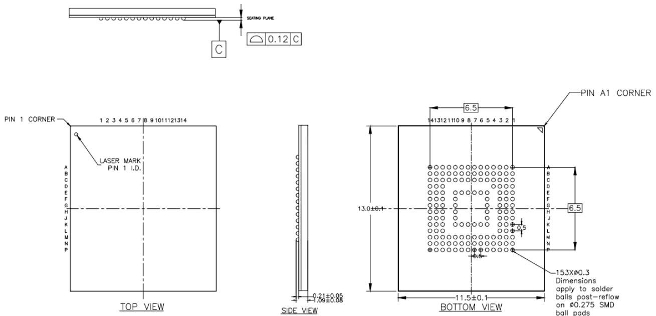
Figure 3.2-1. Package Dimension
