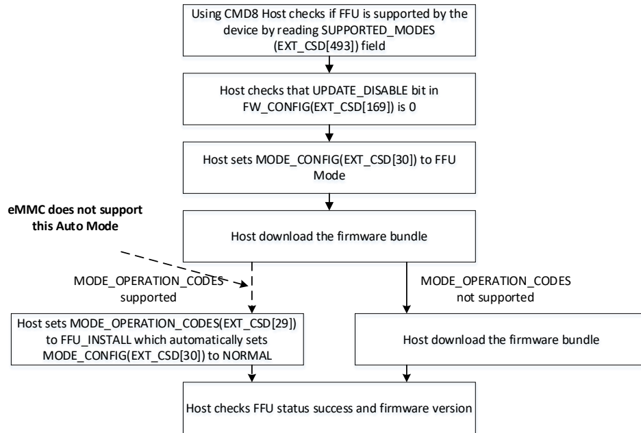
Figure 4.6-1. FFU Flow
