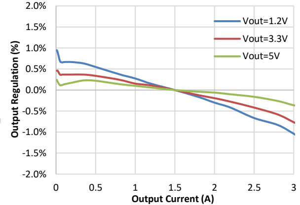
Load Regulation at V_{IN} = 12V V_{IN} = 12V, T_A = 25^\circ C
