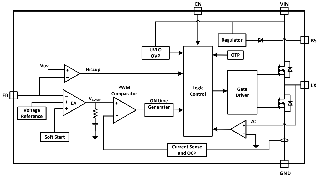
Figure 1. MP1657GTF-Z-MS Block Diagram
