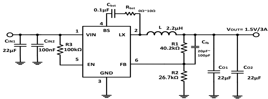
Figure 7. 12V IN , 1.5V/3A Output (V REF =0.6V)
