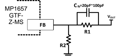
Figure 2. Feedback Network
