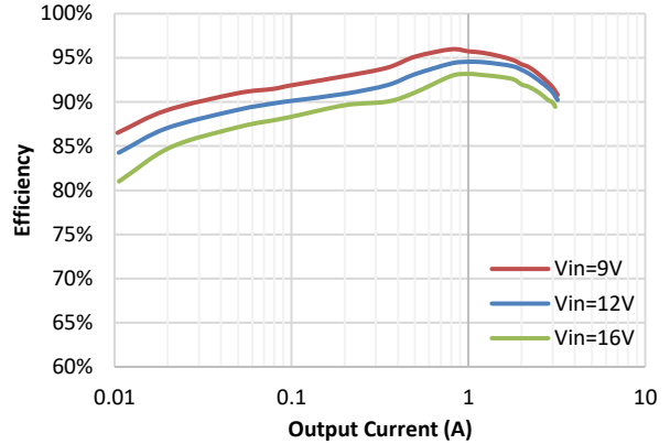
Efficiency at V_{OUT} = 5V V_{OUT} = 5V, L = 4.7\mu H, DCR = 30m\Omega
