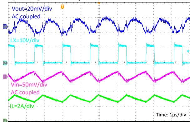
V_{IN} = 12V, V_{OUT} = 3.3V, I_o = 3A
