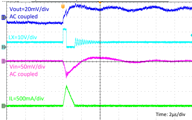
V_{IN} = 12V, V_{OUT} = 3.3V, \text{No Load}
