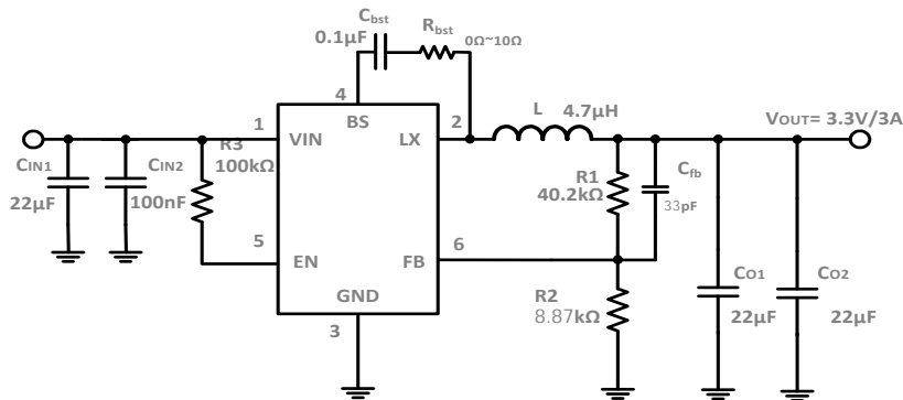
Figure 1. Typical Application of MP1657GTF-Z-MS( V_{REF}=0.6V )
