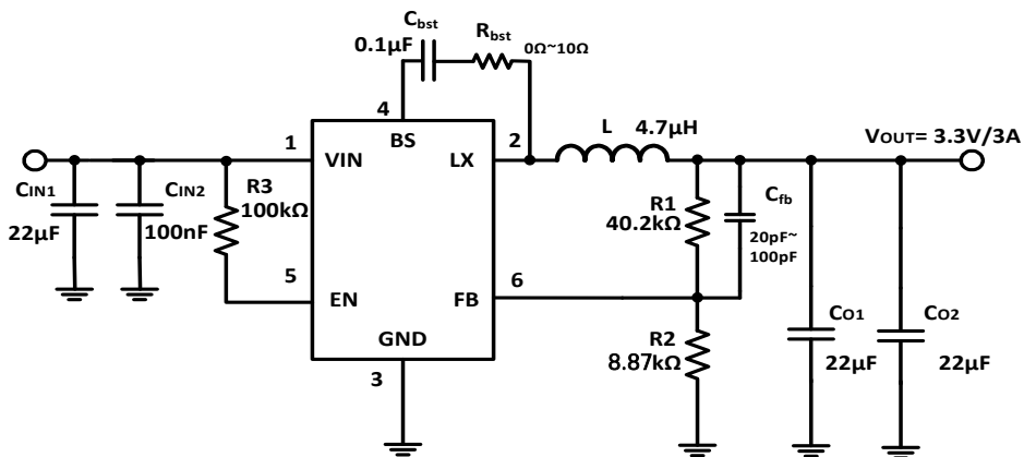
Figure 5. 12V IN , 3.3V/3A Output (V REF =0.6V)
