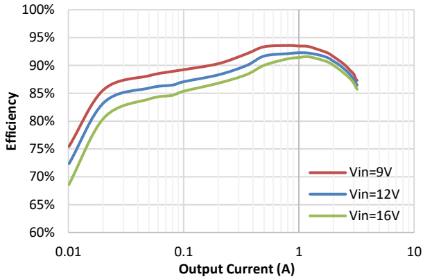
Efficiency at V_{OUT} = 3.3V V_{OUT} = 3.3V, L = 4.7\mu H, DCR = 30m\Omega
