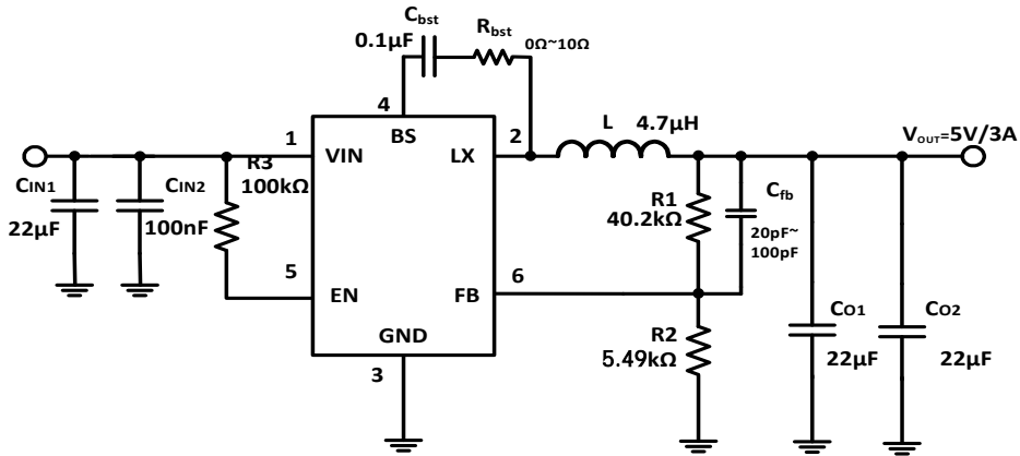
Figure 4. 12V IN , 5V/3A Output (V REF =0.6V)
