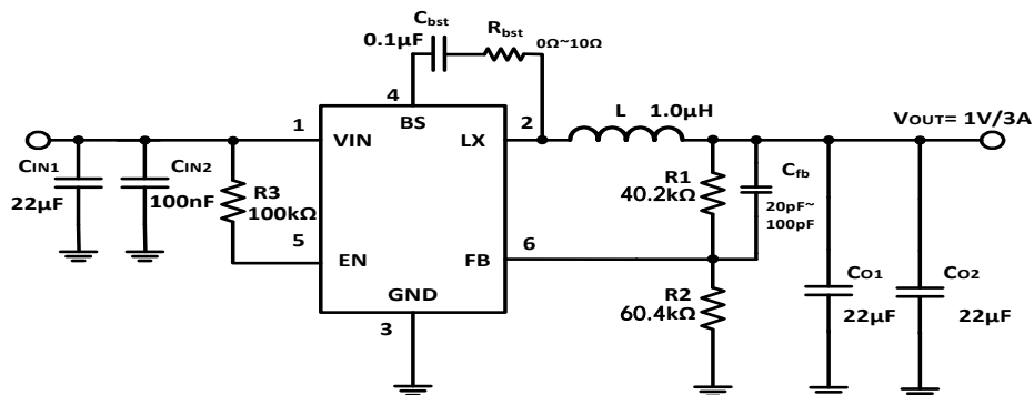
Figure 9. 12V IN , 1V/3A Output (V REF =0.6V)
