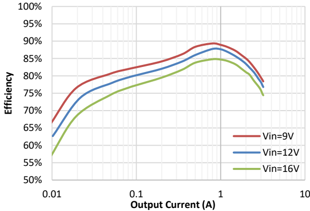
Efficiency at V_{OUT} = 1.2V V_{OUT} = 1.2V, L = 2.2\mu H, DCR = 20m\Omega
