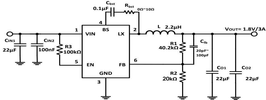
Figure 6. 12V IN , 1.8V/3A Output (V REF =0.6V)
