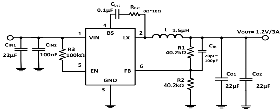
Figure 8. 12V IN , 1.2V/3A Output (V REF =0.6V)
