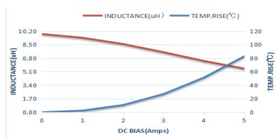
MTQH707015S100MBT
