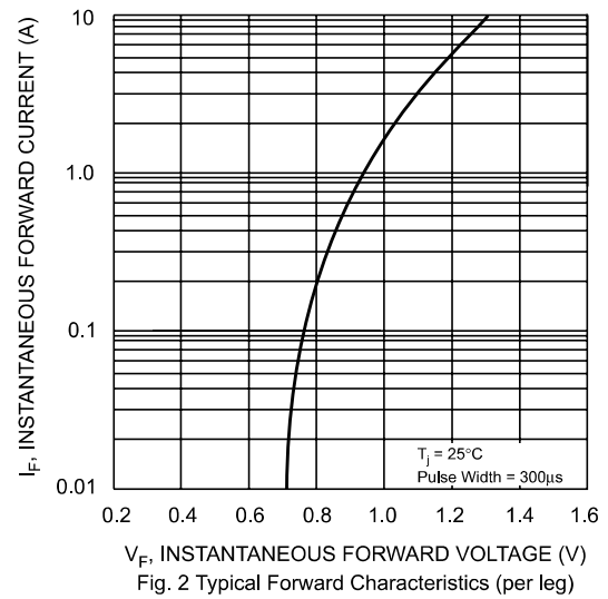
Fig. 2 Typical Forward Characteristics (per leg)
