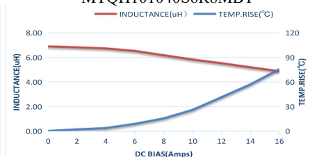
MTQH101040S6R8MBT
