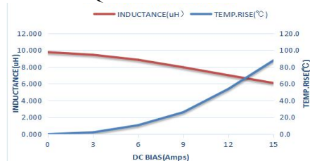
MTQH101040S100MBT
