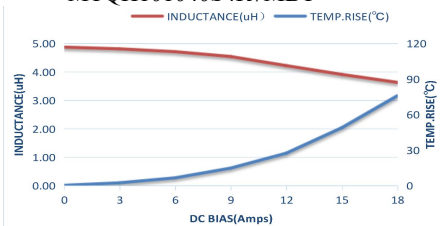
MTQH101040S4R7MBT
