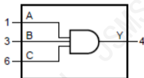
Figure 1. Logic symbol
