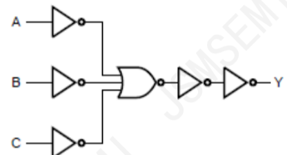
Figure 3. Logic diagram
