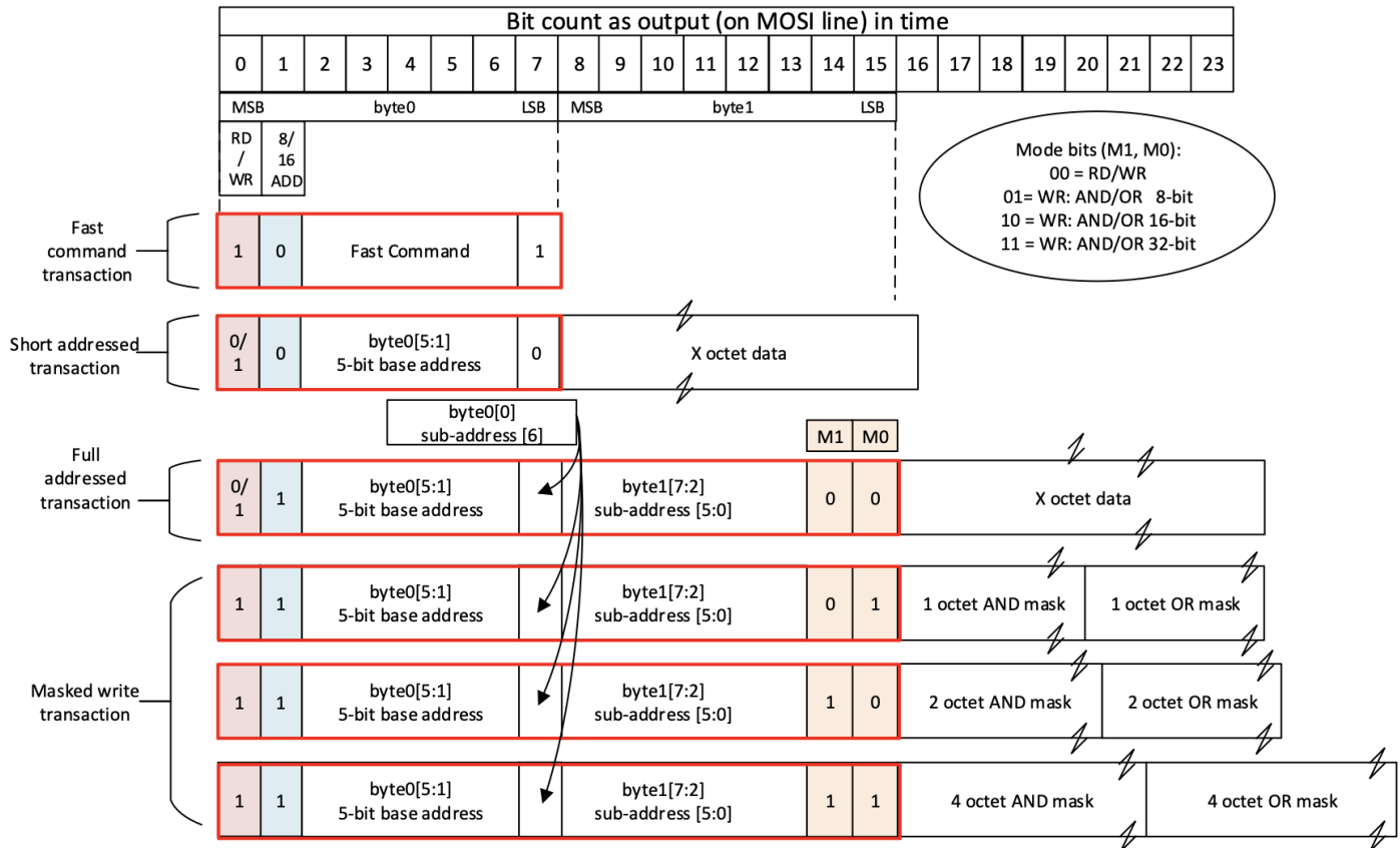
Figure 9: SPI Command Formatting
