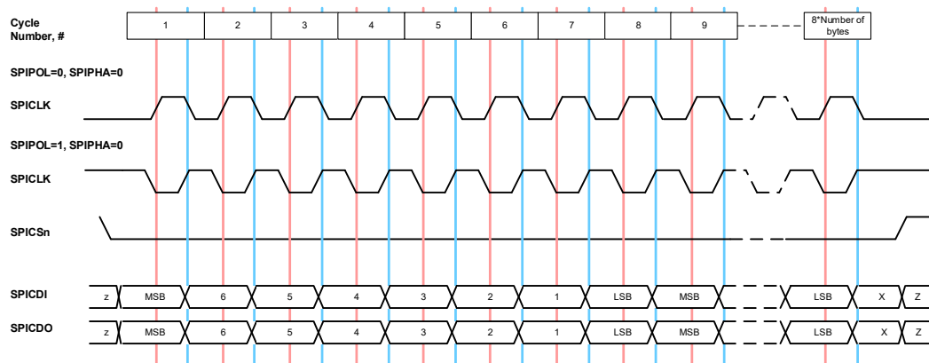
Figure 7: QM33120W SPIPHA=0 Transfer Protocol
