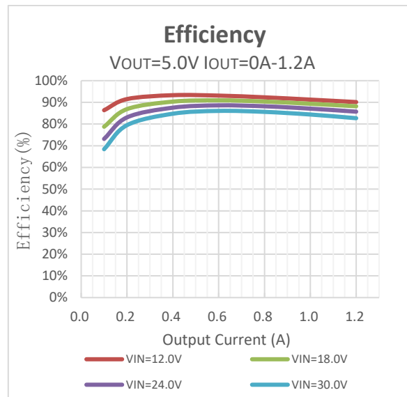
Efficiency V_{OUT}=5V
