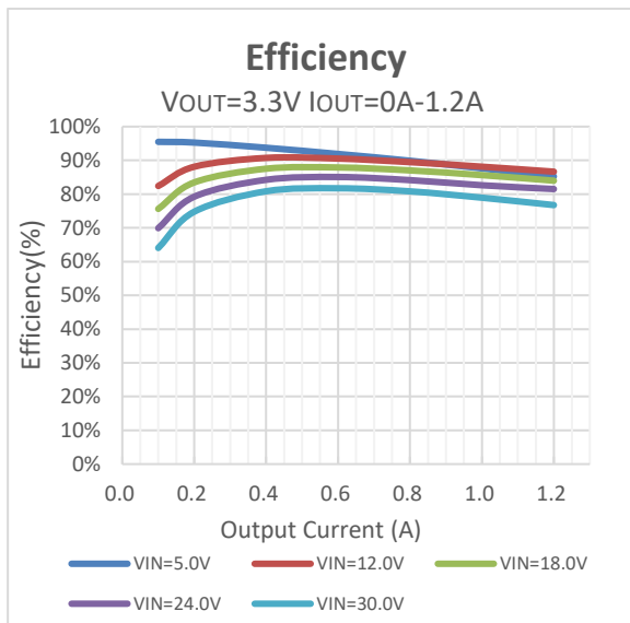
Efficiency V_{OUT}=3.3V
