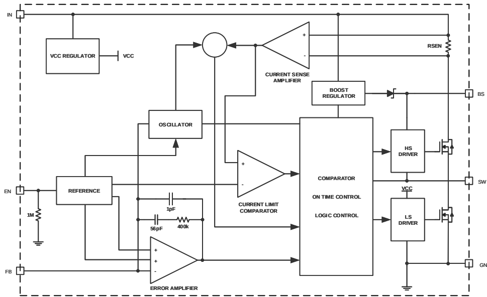
R1244N001B-TR-FE-MS Block Diagram
