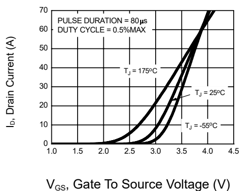
Figure 5: Transfer Characteristics
