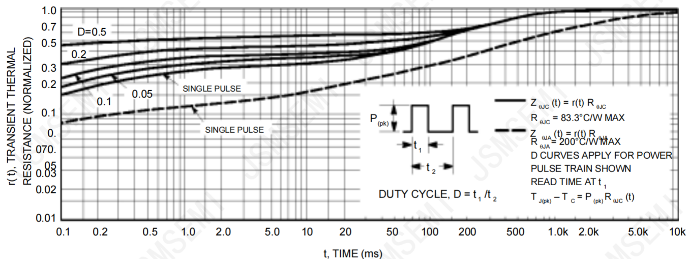
Figure 13. Thermal Response
