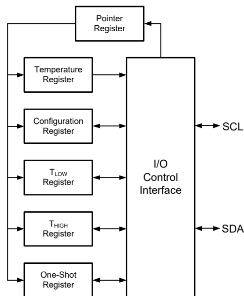
Figure 5. Internal Register Structure
