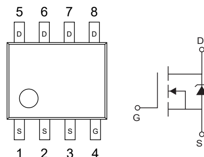
SOP-8
