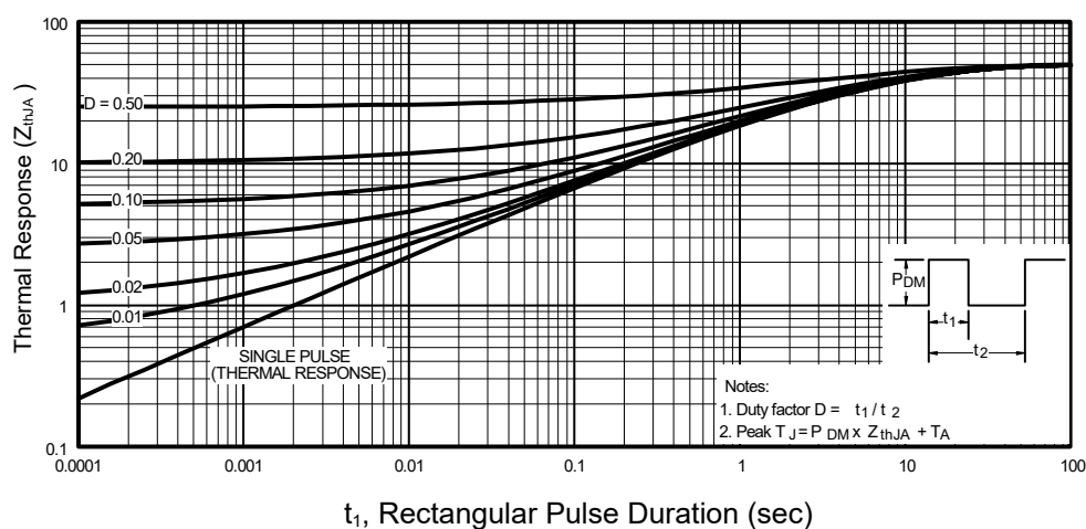
Fig 10. Maximum Effective Transient Thermal Impedance, Junction-to-Ambient
