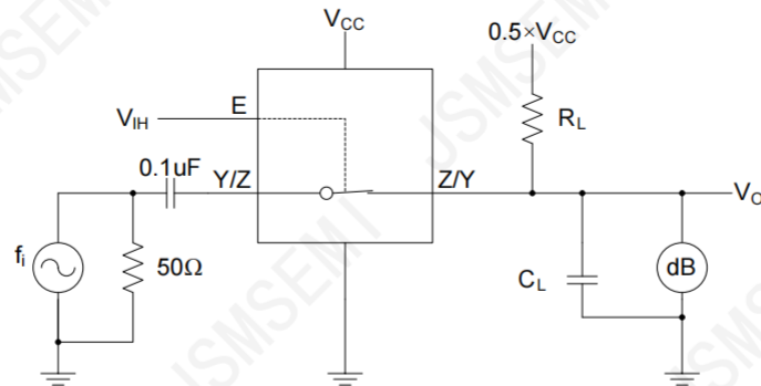
Figure 11. Test circuit for measuring the frequency response when switch is in ON-state
