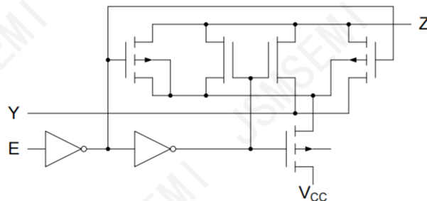
Figure 3. Logic diagram
