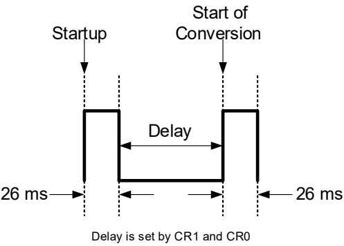
Figure 3. Schematic Diagram of Continuous Conversion
