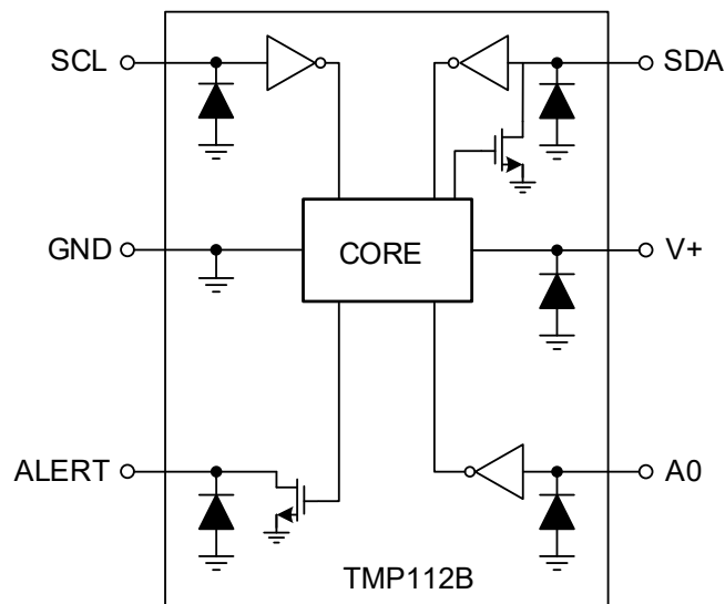
Figure 2. TMP112B Internal ESD Equivalent Circuit
