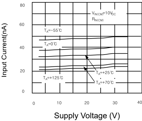
Figure 1: Input Current versus Supply Voltage
