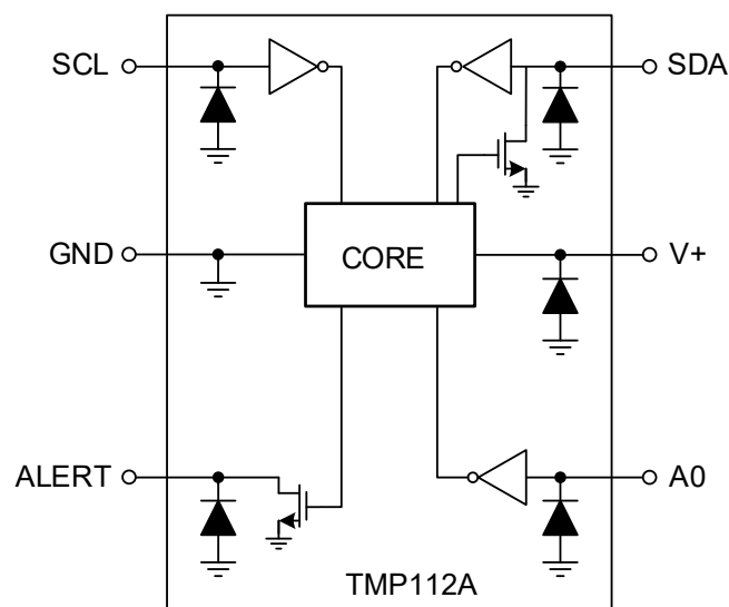
Figure 2. TMP112A Internal ESD Equivalent Circuit
