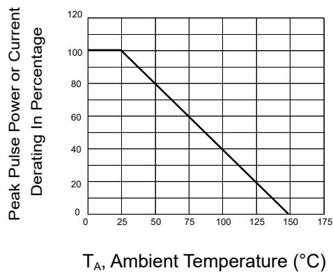
Figure 1: Pulse Derating Curve
