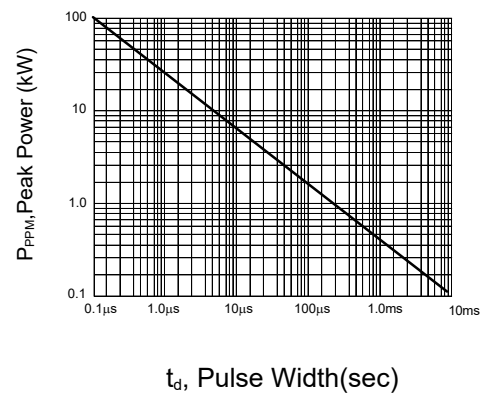
Figure 4: Peak Pulse Power Rating Curve
