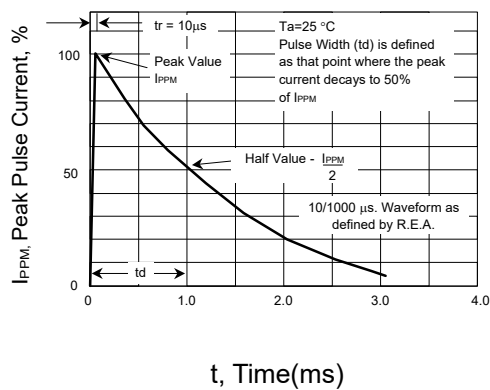
Figure 3: Pulse Waveform
