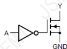
Figure 3. Logic diagram (one driver)
