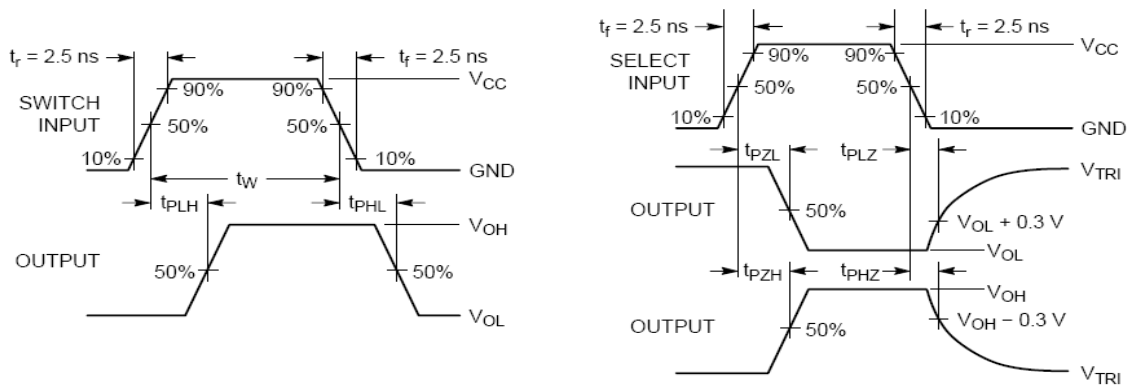
Figure 1: Transmission delay
