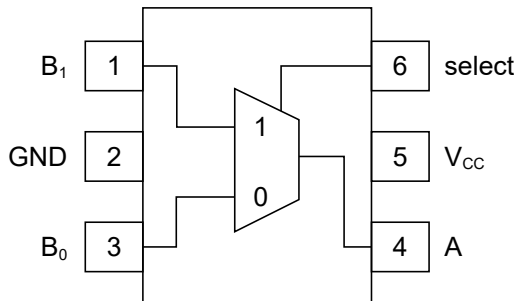
SC70-6/SOT23-6
