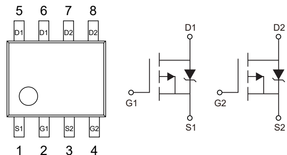
SOP-8
