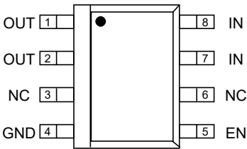
MIC5200-x.xYM (SOP-8)
