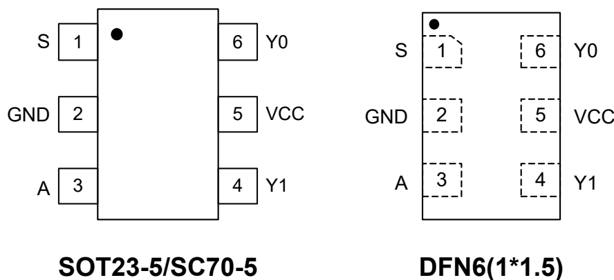
Figure1. Top View
