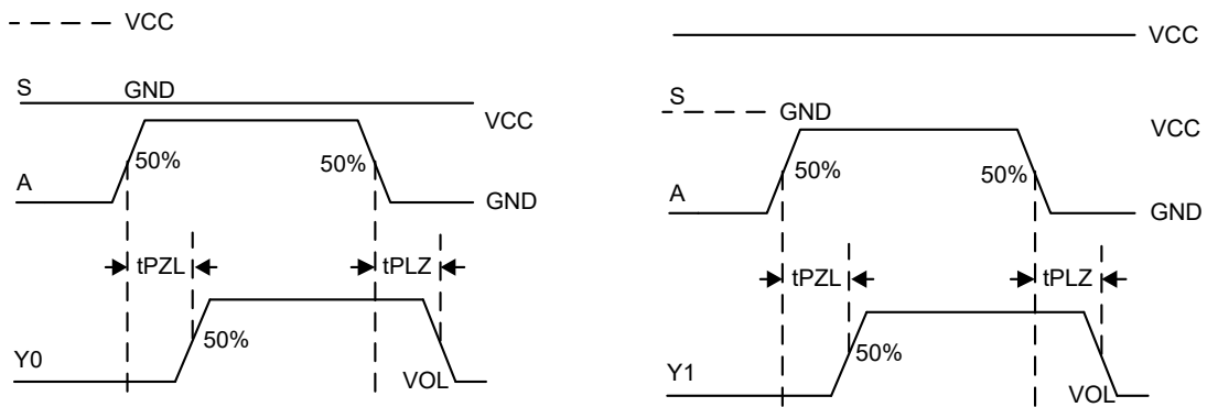
Figure3. Switching Waveforms
