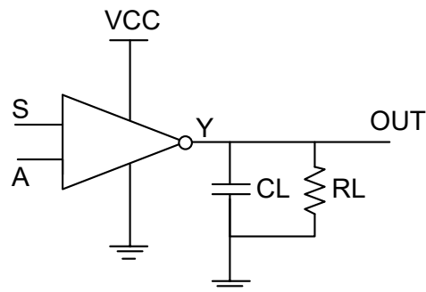
Figure4. Test Circuit
