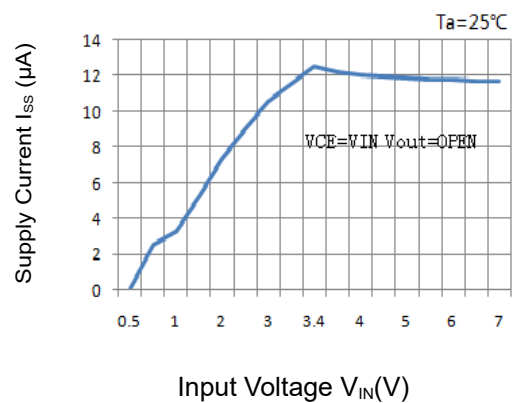
Figure 4: Input voltage and static current
