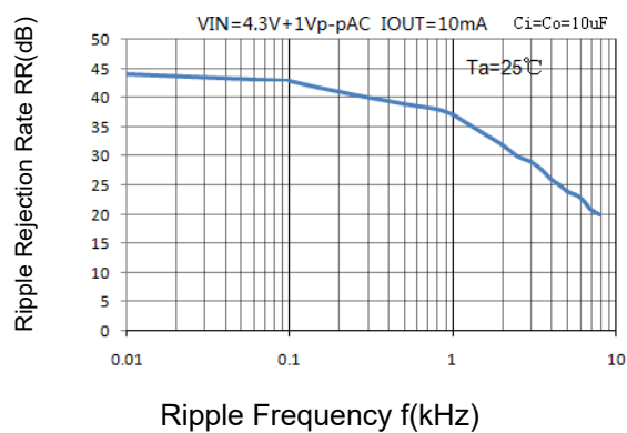
Figure 5: Ripple suppression
