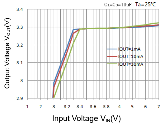
Figure 2: Output voltage and input voltage
