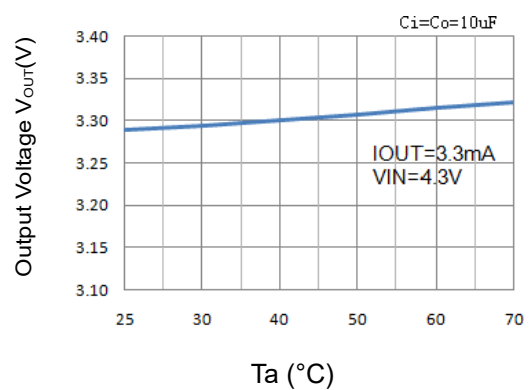
Figure 6: Output voltage and temperature
