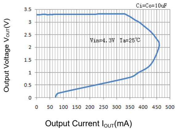
Figure 1: Output voltage and output current
