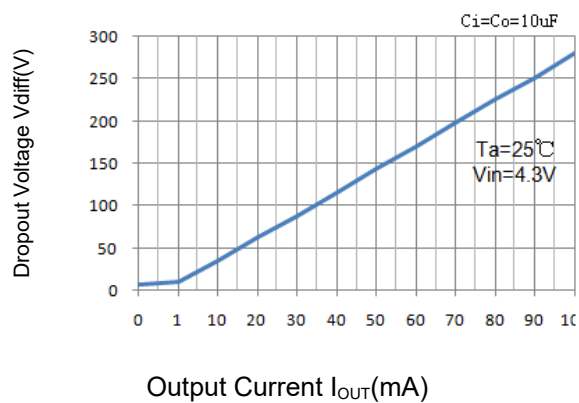
Figure 3: Dropout voltage and output current
