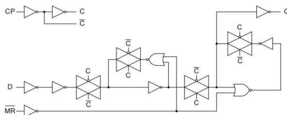
Figure 2. Logic diagram
