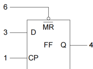
Figure 1. Logic symbol
